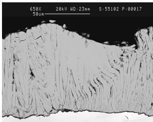
Fig. 5 Cross-sectional secondary electron image of an EB-PVD top coat that has undergone impact damage during engine operation. (Image is courtesy of R. Darolia at General Electric Transportation.)
